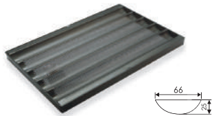
Al. Alloy 5 Rows Baguette Tray (Non-Stick)
